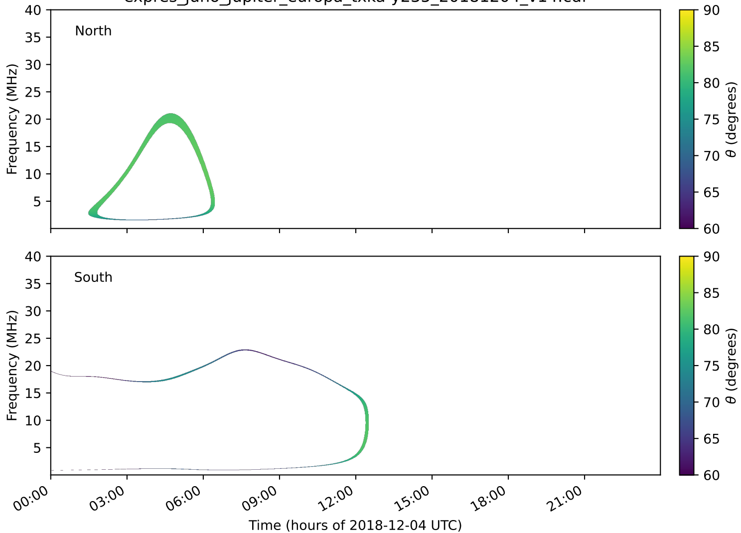
expres_juno_jupiter_europa_txka-y235_20181204_v14.cdf
