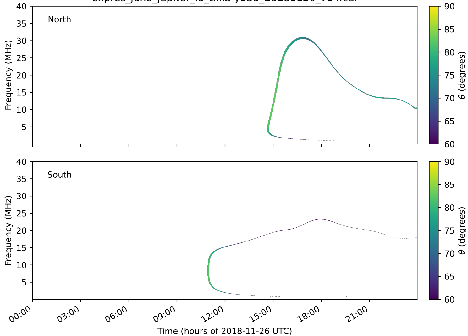
expres_juno_jupiter_io_txka-y235_20181126_v14.cdf
