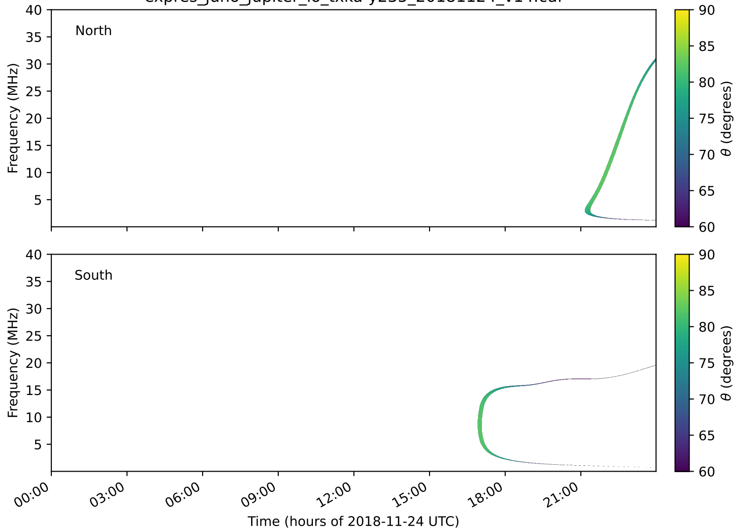
expres_juno_jupiter_io_txka-y235_20181124_v14.cdf
