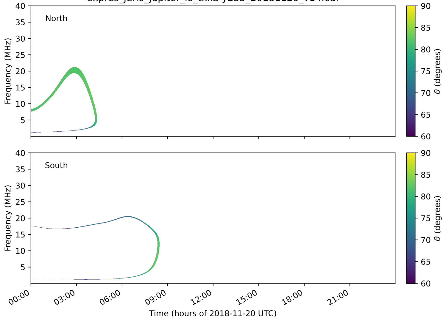
expres_juno_jupiter_io_txka-y235_20181120_v14.cdf
