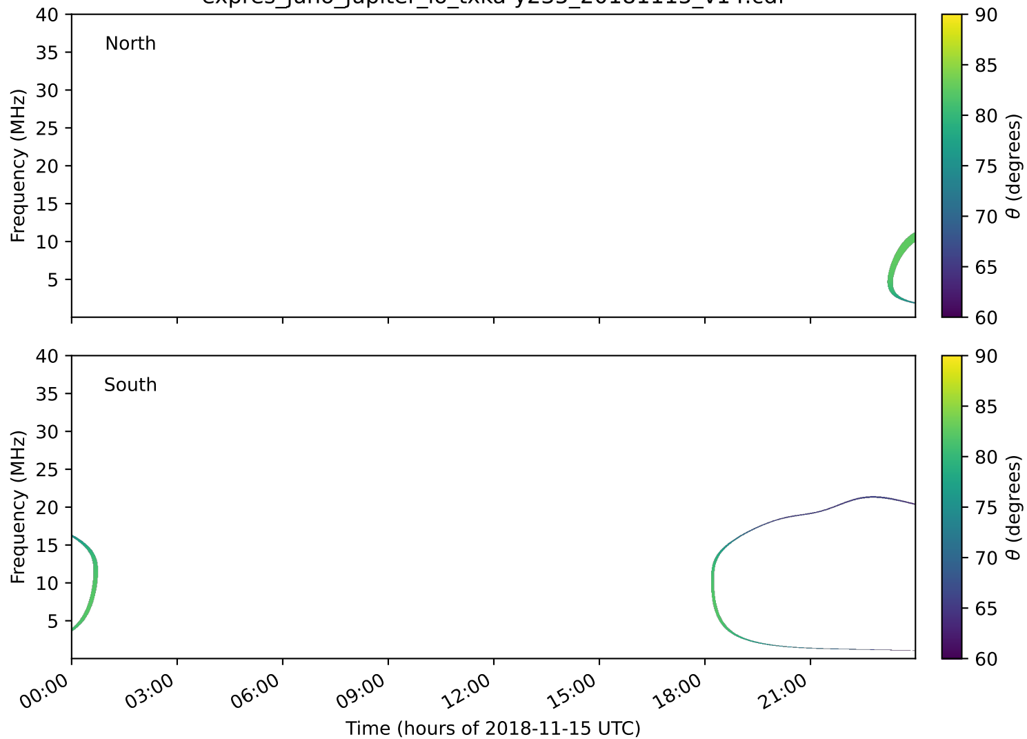
expres_juno_jupiter_io_txka-y235_20181115_v14.cdf
