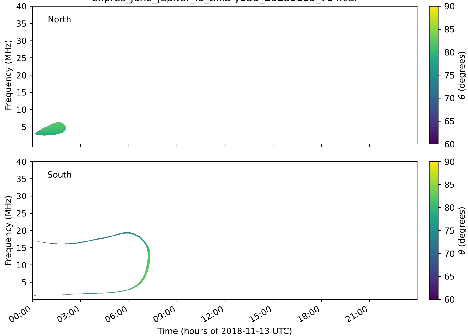
expres_juno_jupiter_io_txka-y235_20181113_v14.cdf
