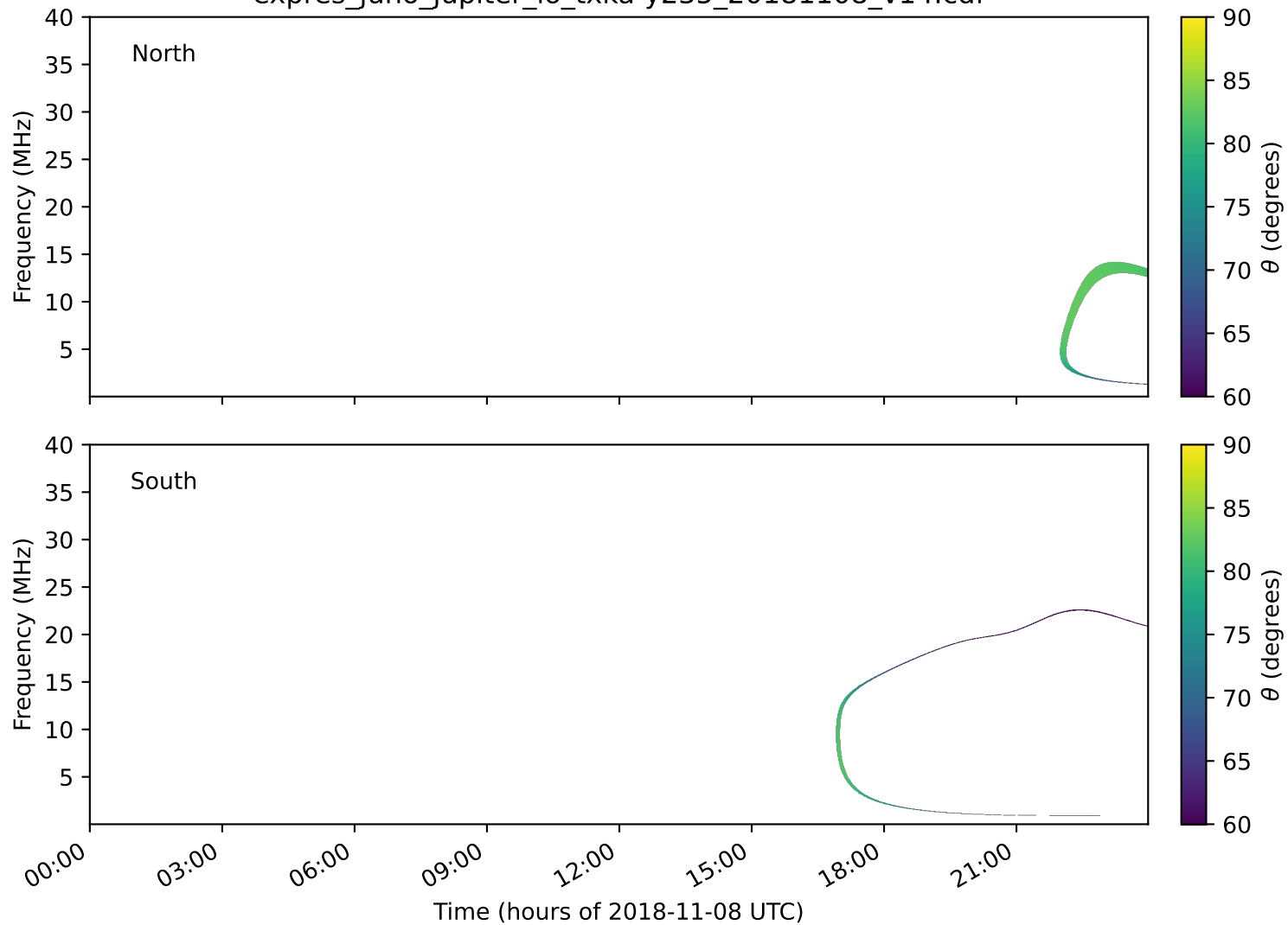
expres_juno_jupiter_io_txka-y235_20181108_v14.cdf
