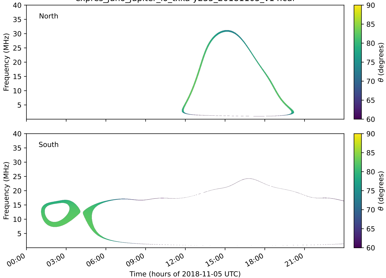
expres_juno_jupiter_io_txka-y235_20181105_v14.cdf
