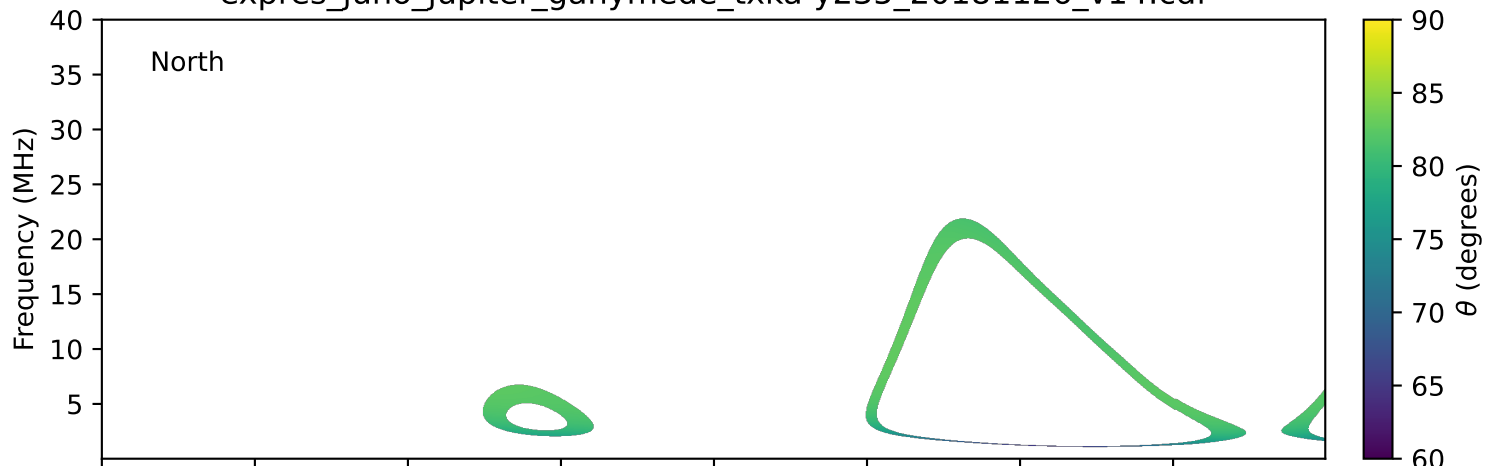
expres_juno_jupiter_ganymede_txka-y235_20181126_v14.cdf
