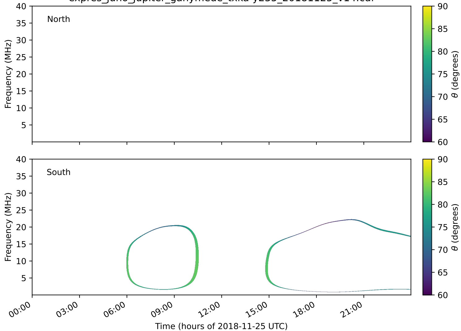
expres_juno_jupiter_ganymede_txka-y235_20181125_v14.cdf
