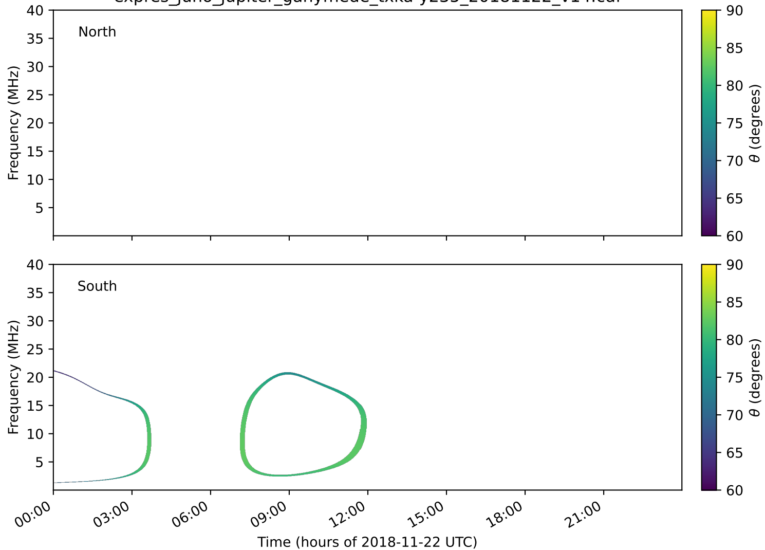
expres_juno_jupiter_ganymede_txka-y235_20181122_v14.cdf
