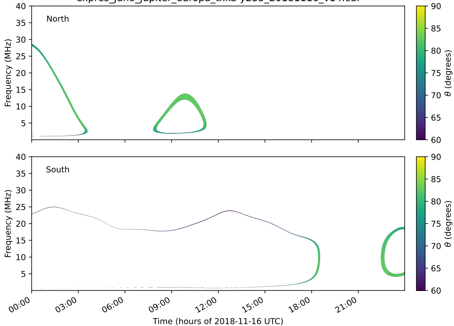
expres_juno_jupiter_europa_txka-y235_20181116_v14.cdf
