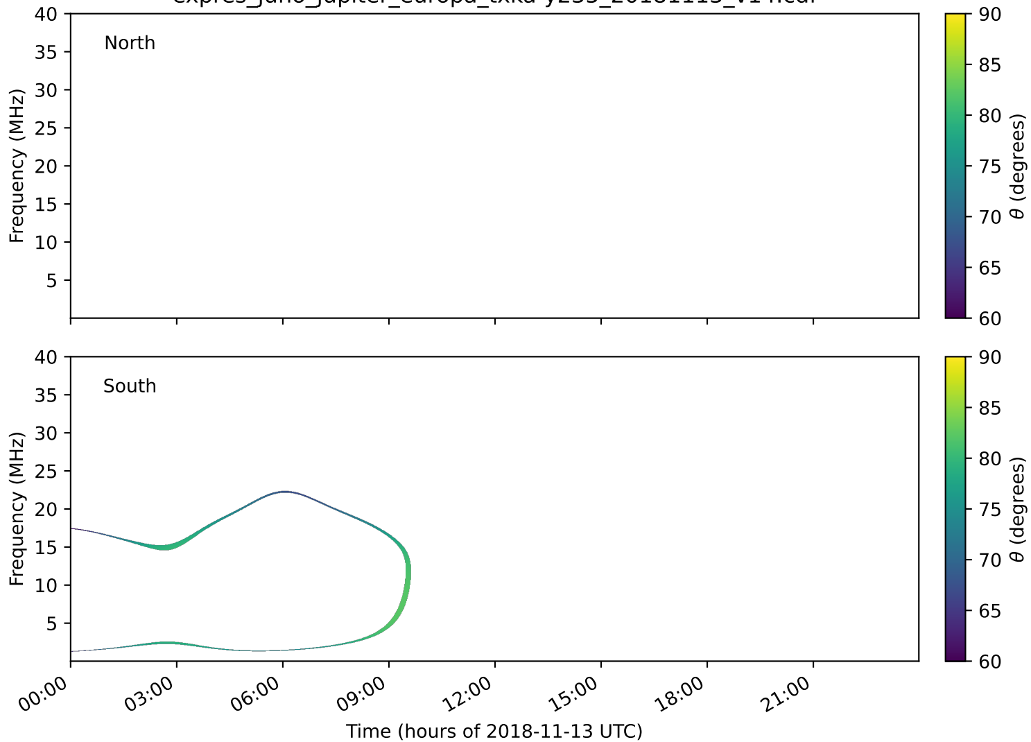
expres_juno_jupiter_europa_txka-y235_20181113_v14.cdf
