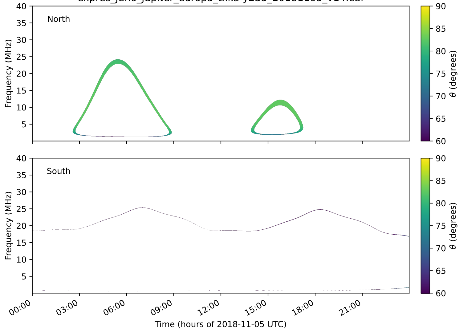
expres_juno_jupiter_europa_txka-y235_20181105_v14.cdf
