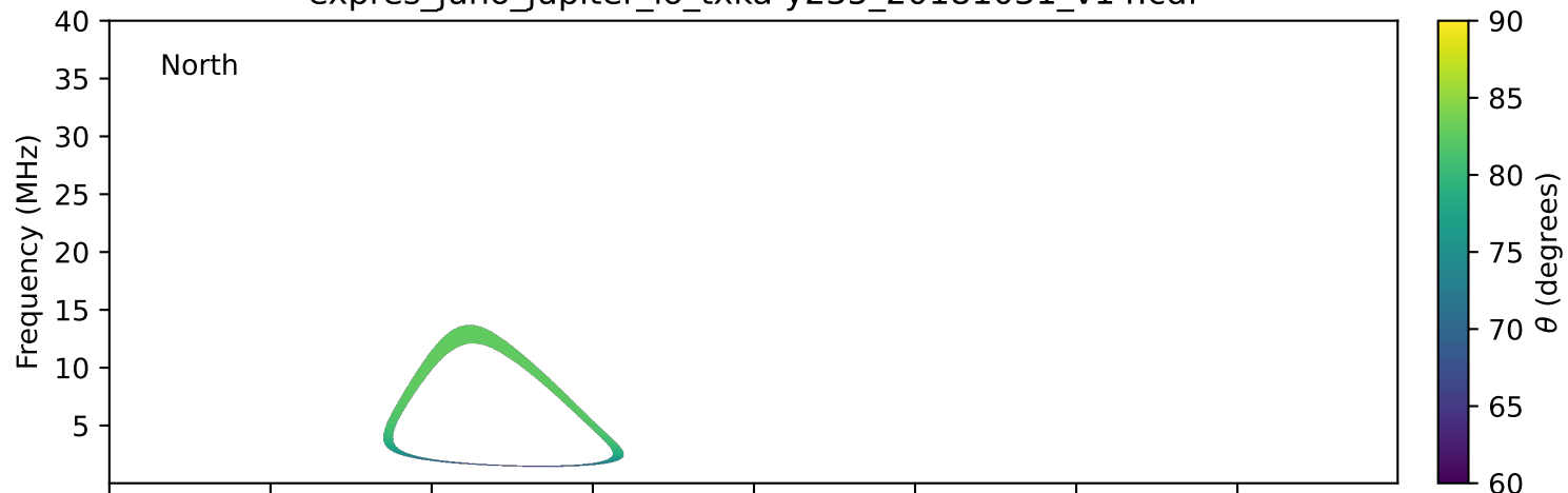
expres_juno_jupiter_io_txka-y235_20181031_v14.cdf
