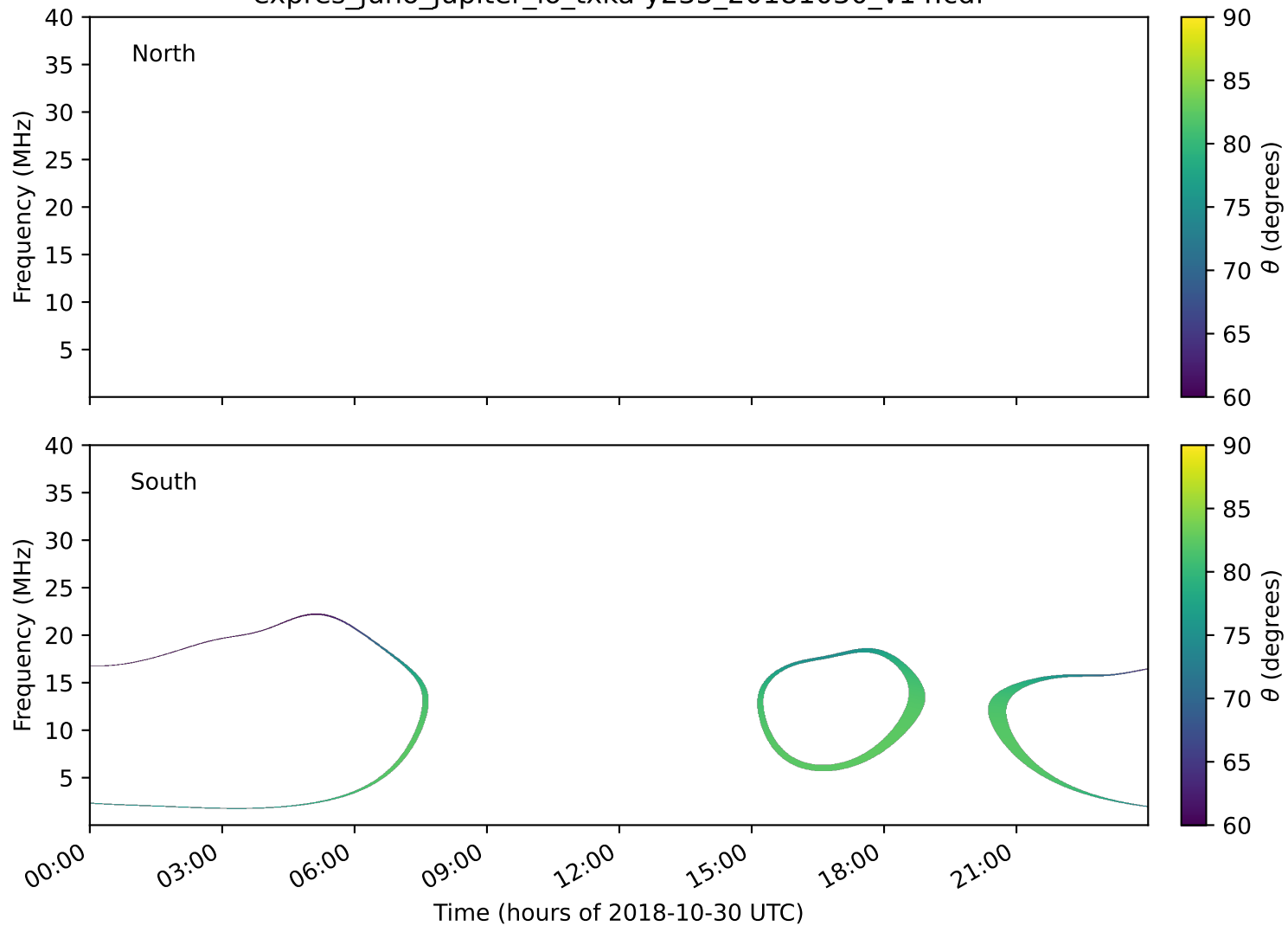
expres_juno_jupiter_io_txka-y235_20181030_v14.cdf
