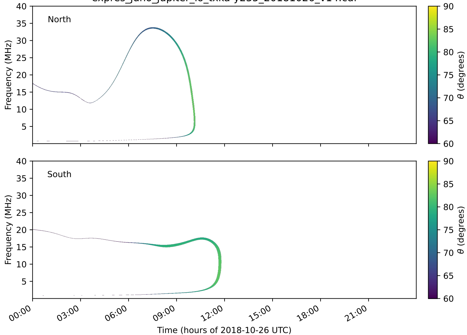
expres_juno_jupiter_io_txka-y235_20181026_v14.cdf
