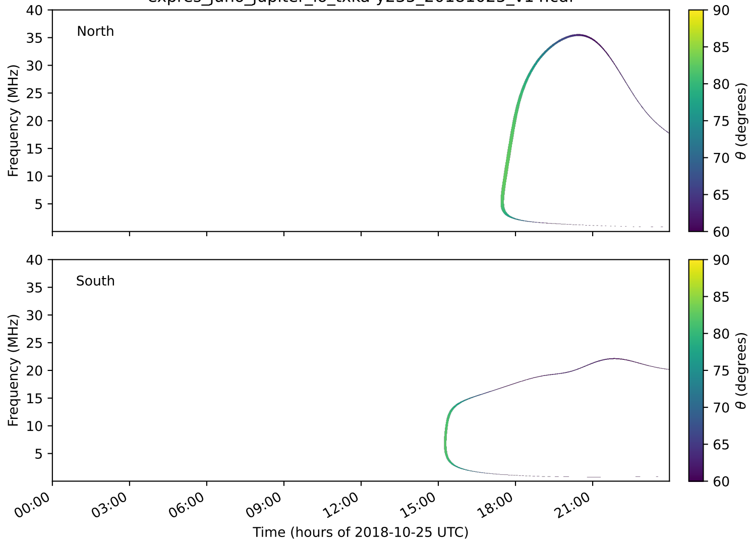
expres_juno_jupiter_io_txka-y235_20181025_v14.cdf
