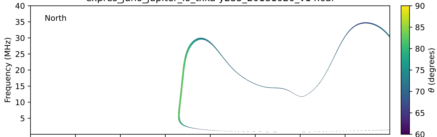
expres_juno_jupiter_io_txka-y235_20181020_v14.cdf
