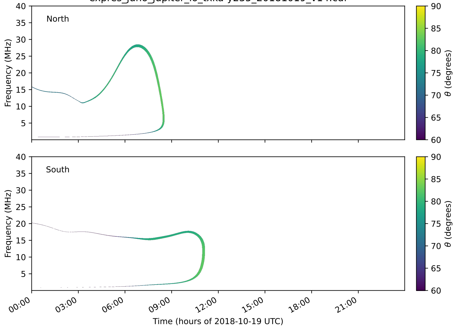
expres_juno_jupiter_io_txka-y235_20181019_v14.cdf
