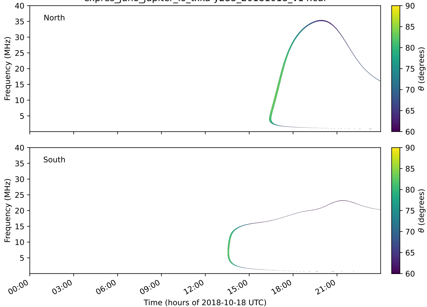
expres_juno_jupiter_io_txka-y235_20181018_v14.cdf
