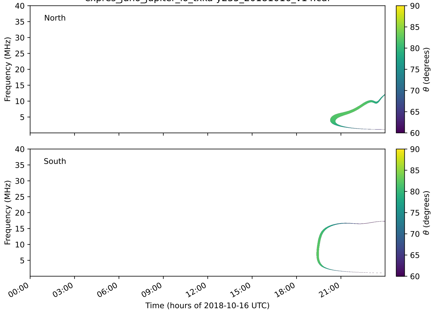
expres_juno_jupiter_io_txka-y235_20181016_v14.cdf
