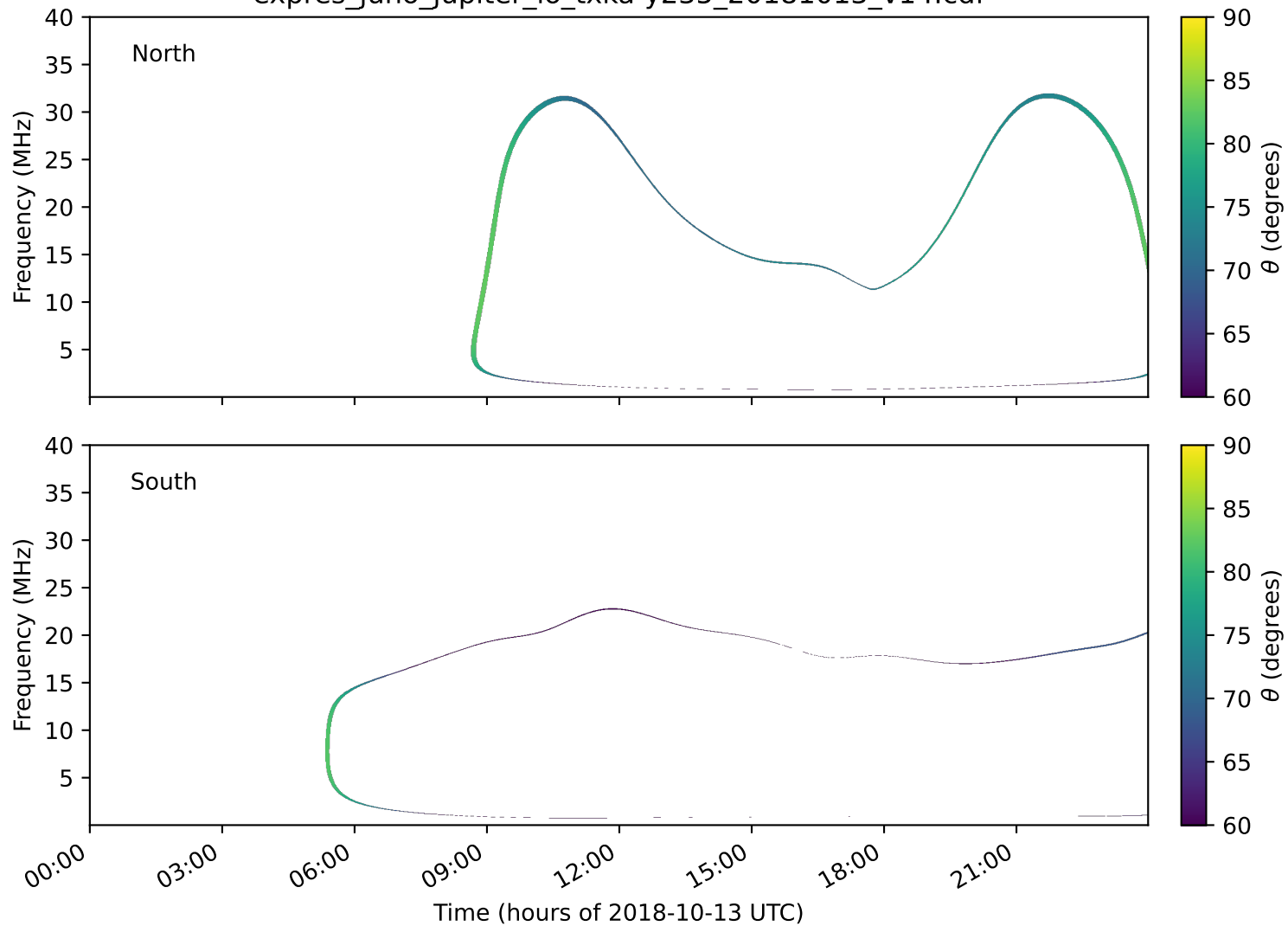
expres_juno_jupiter_io_txka-y235_20181013_v14.cdf
