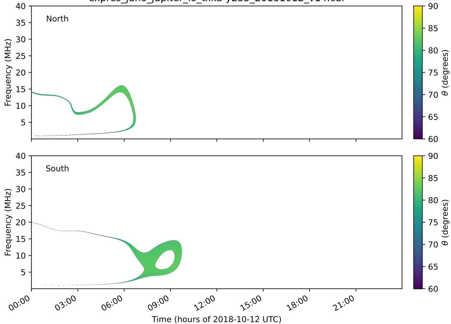
expres_juno_jupiter_io_txka-y235_20181012_v14.cdf
