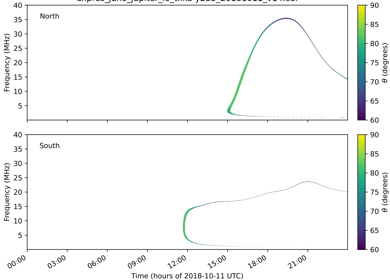
expres_juno_jupiter_io_txka-y235_20181011_v14.cdf
