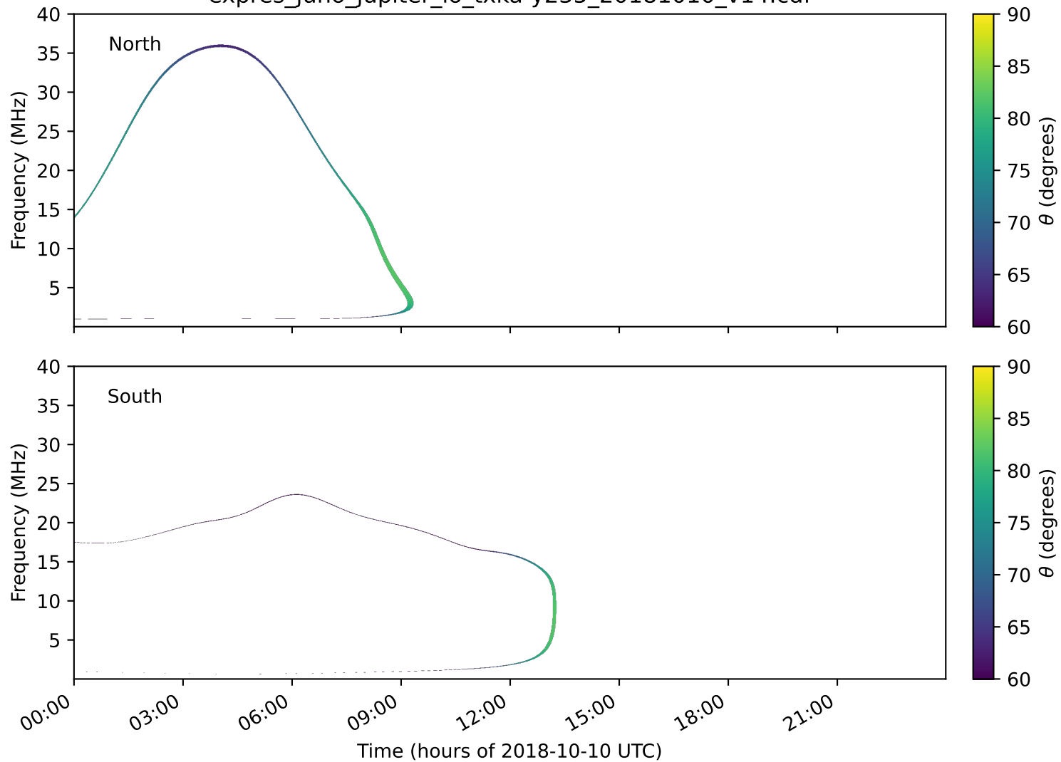
expres_juno_jupiter_io_txka-y235_20181010_v14.cdf
