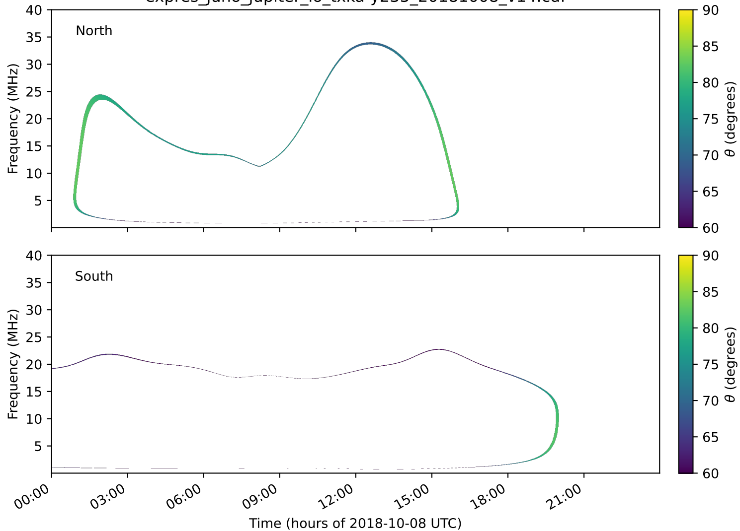
expres_juno_jupiter_io_txka-y235_20181008_v14.cdf
