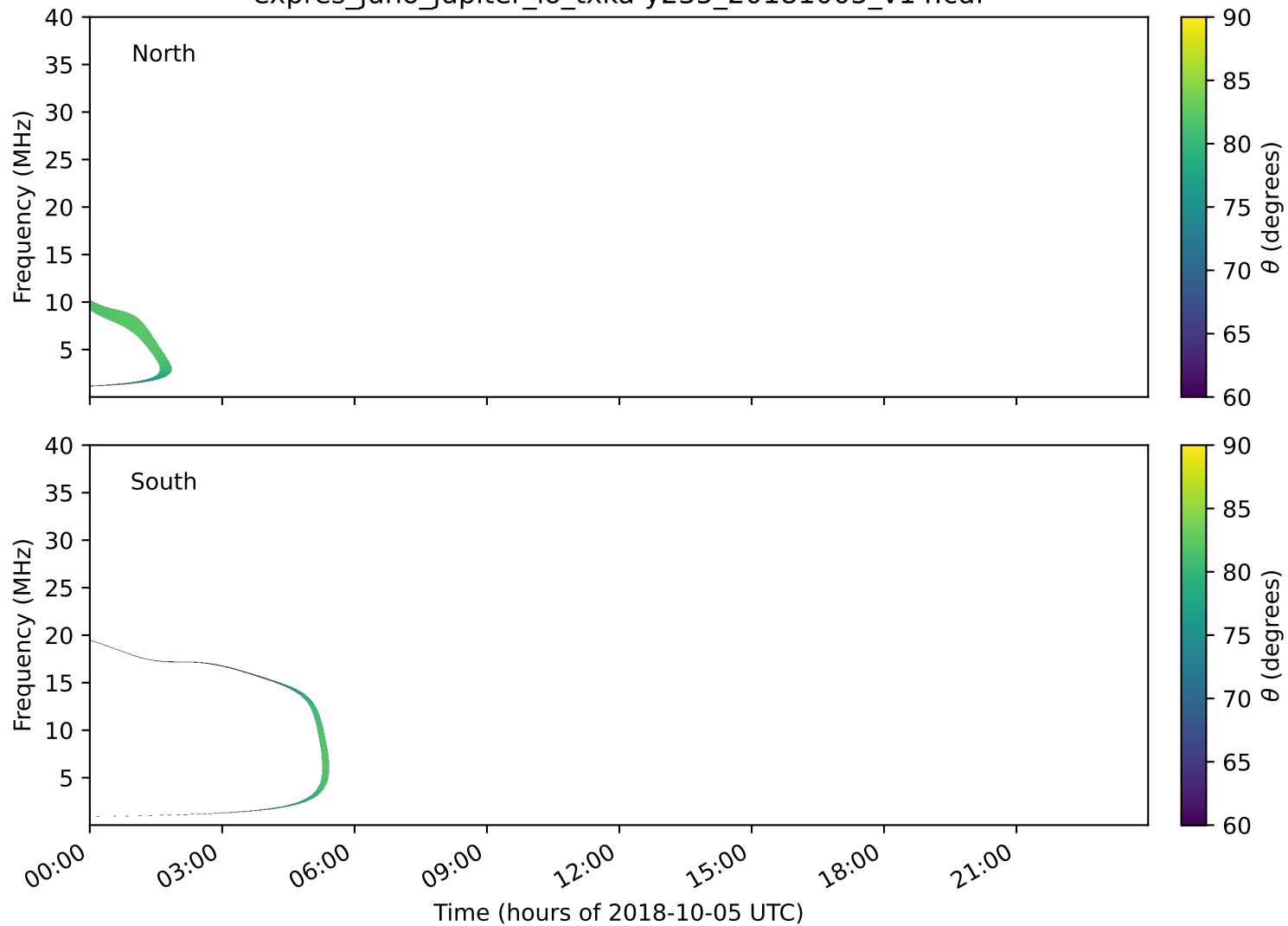
expres_juno_jupiter_io_txka-y235_20181005_v14.cdf
