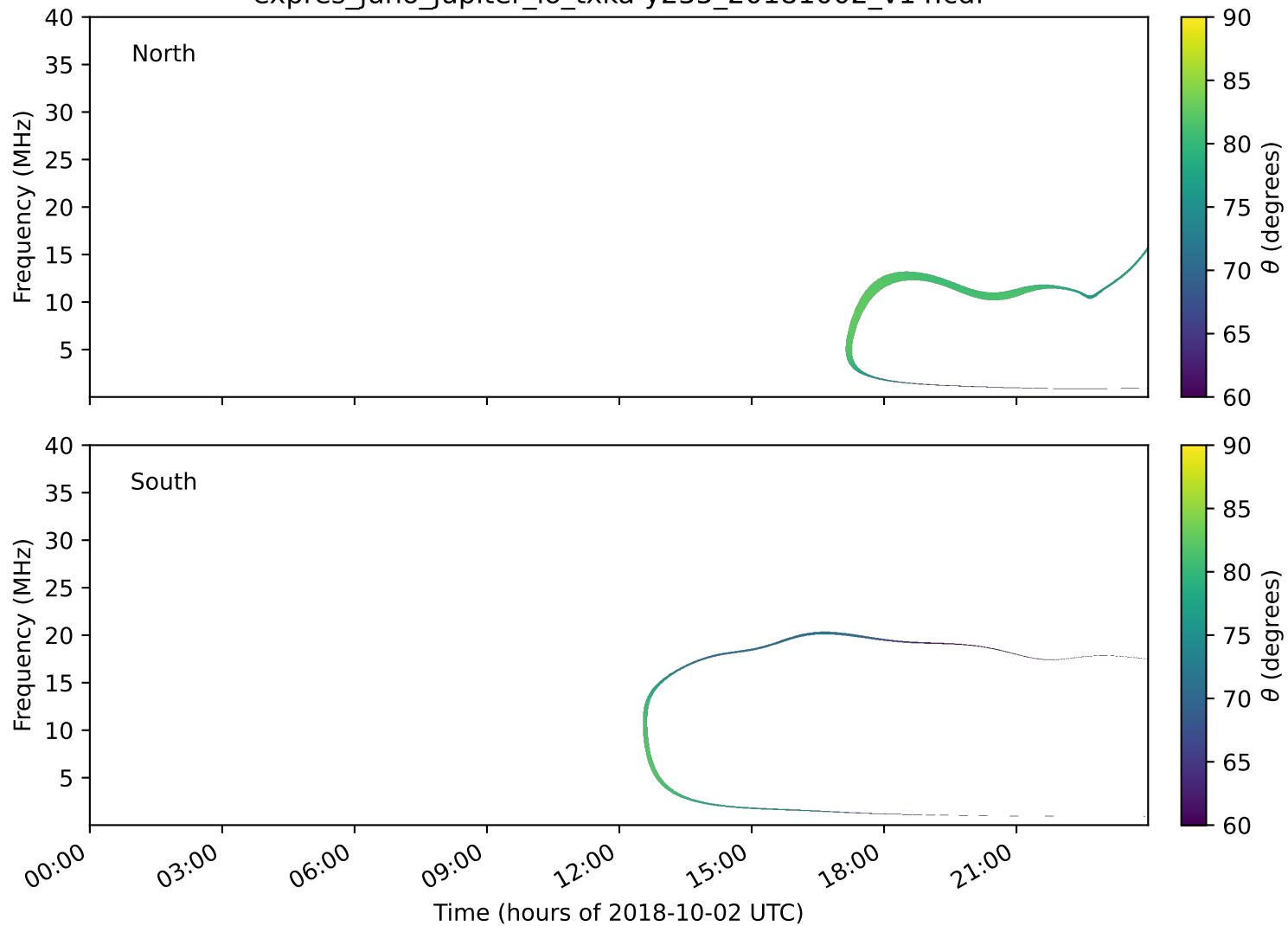
expres_juno_jupiter_io_txka-y235_20181002_v14.cdf
