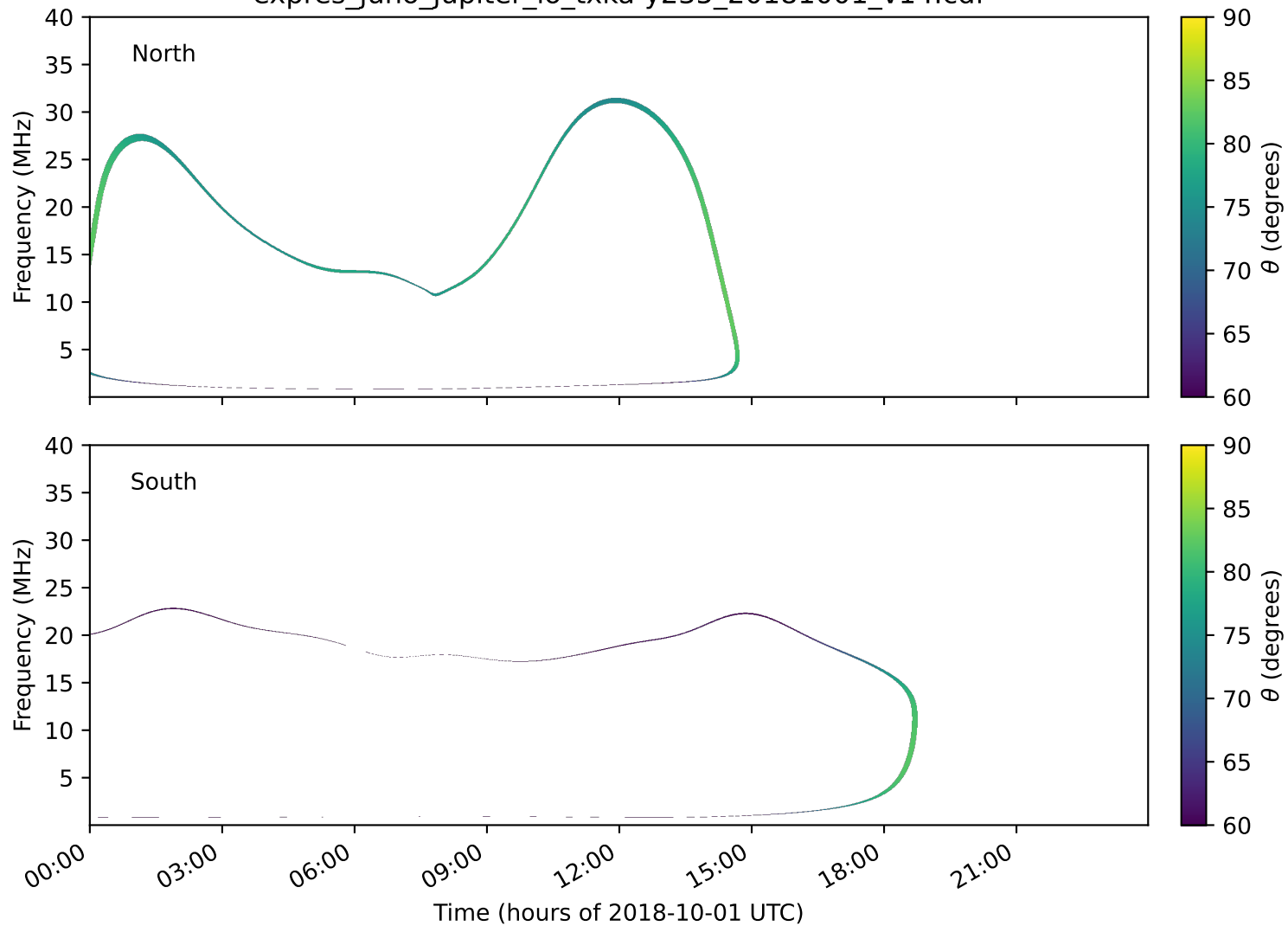
expres_juno_jupiter_io_txka-y235_20181001_v14.cdf
