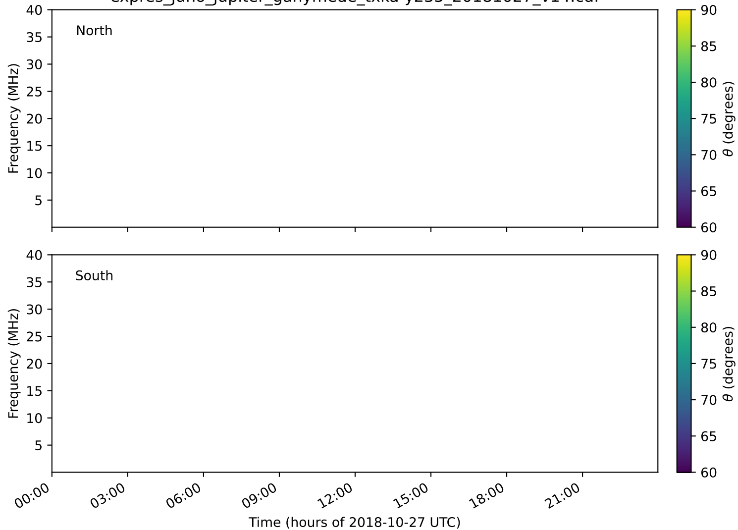
expres_juno_jupiter_ganymede_txka-y235_20181027_v14.cdf
