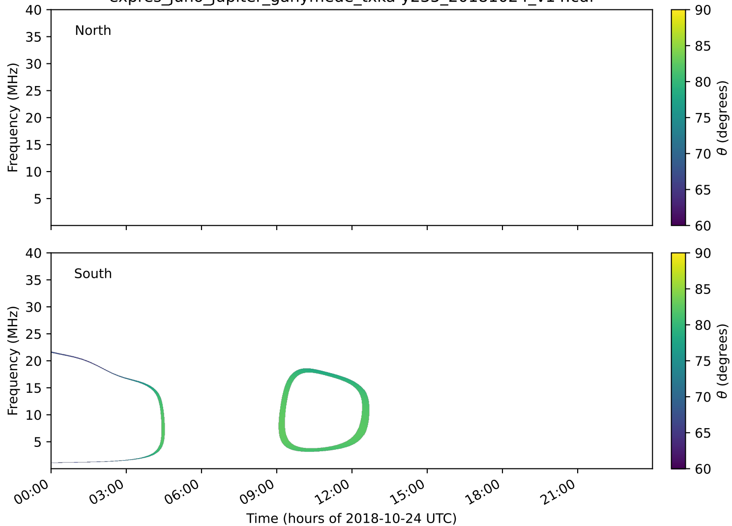
expres_juno_jupiter_ganymede_txka-y235_20181024_v14.cdf
