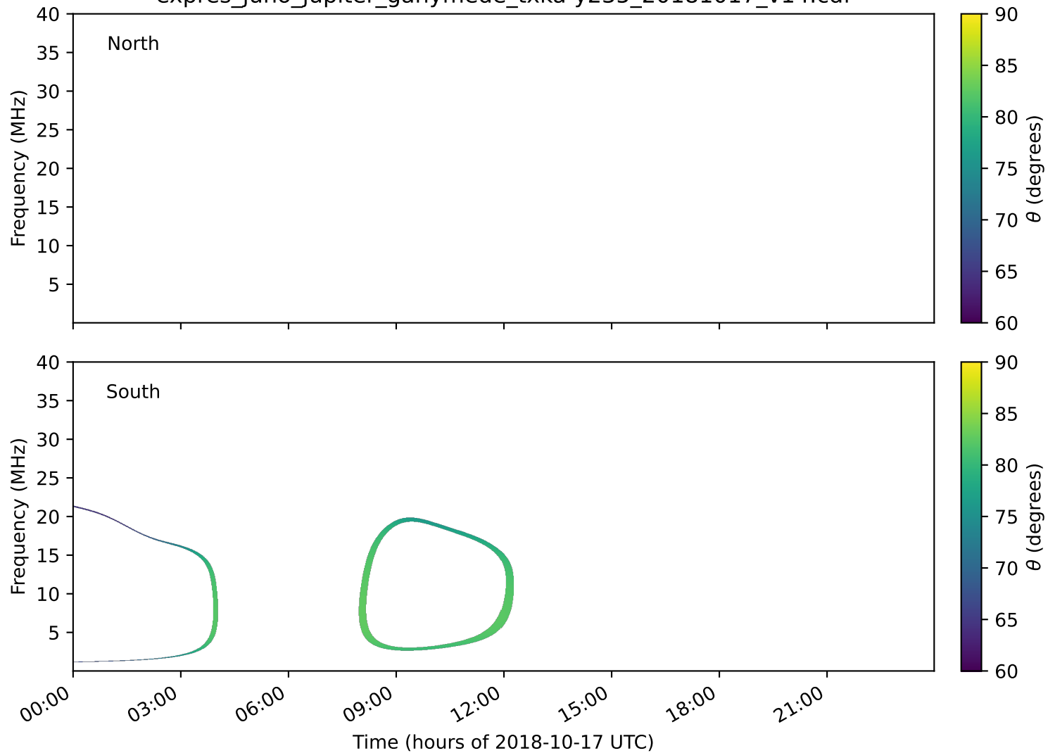
expres_juno_jupiter_ganymede_txka-y235_20181017_v14.cdf
