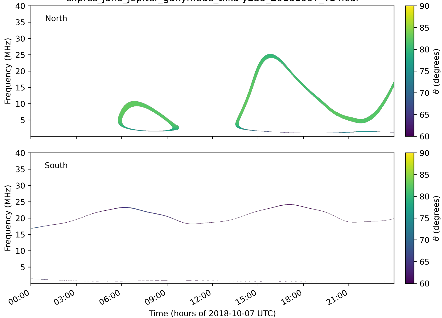
expres_juno_jupiter_ganymede_txka-y235_20181007_v14.cdf
