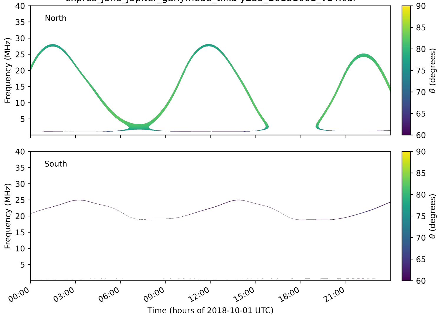
expres_juno_jupiter_ganymede_txka-y235_20181001_v14.cdf
