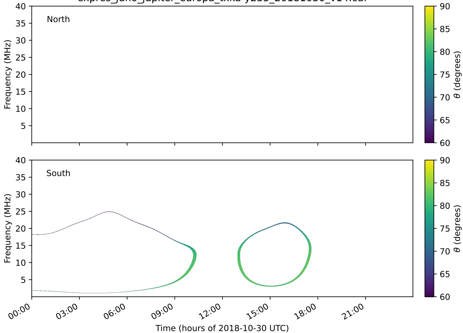
expres_juno_jupiter_europa_txka-y235_20181030_v14.cdf
