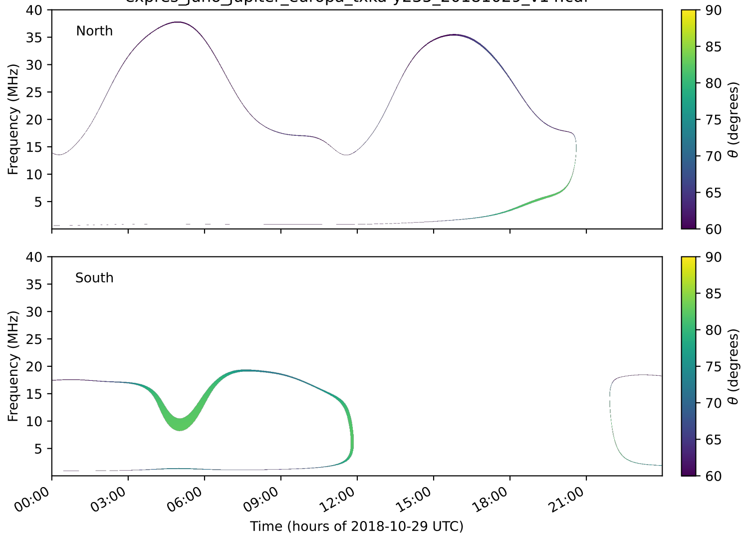
expres_juno_jupiter_europa_txka-y235_20181029_v14.cdf
