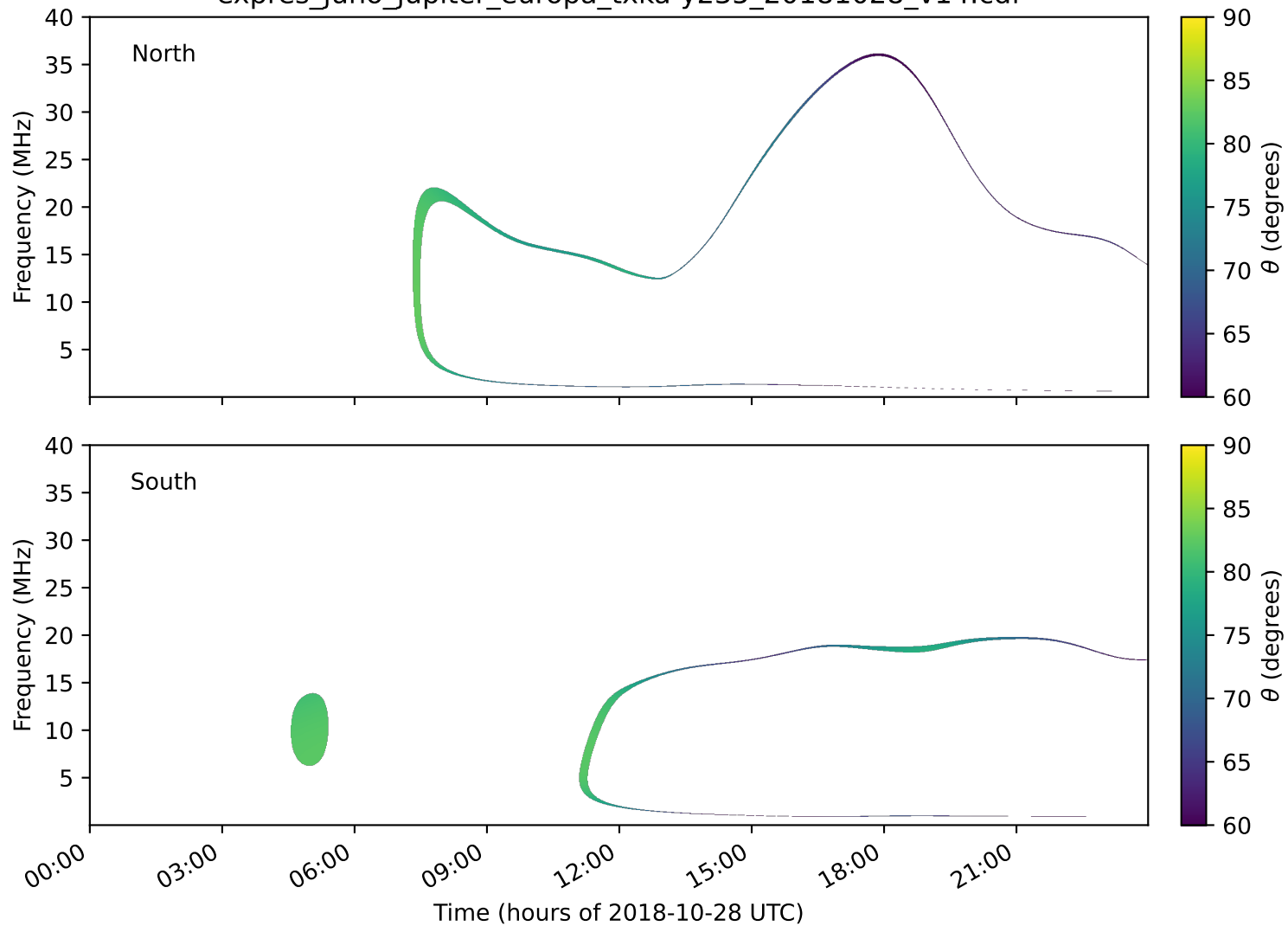
expres_juno_jupiter_europa_txka-y235_20181028_v14.cdf
