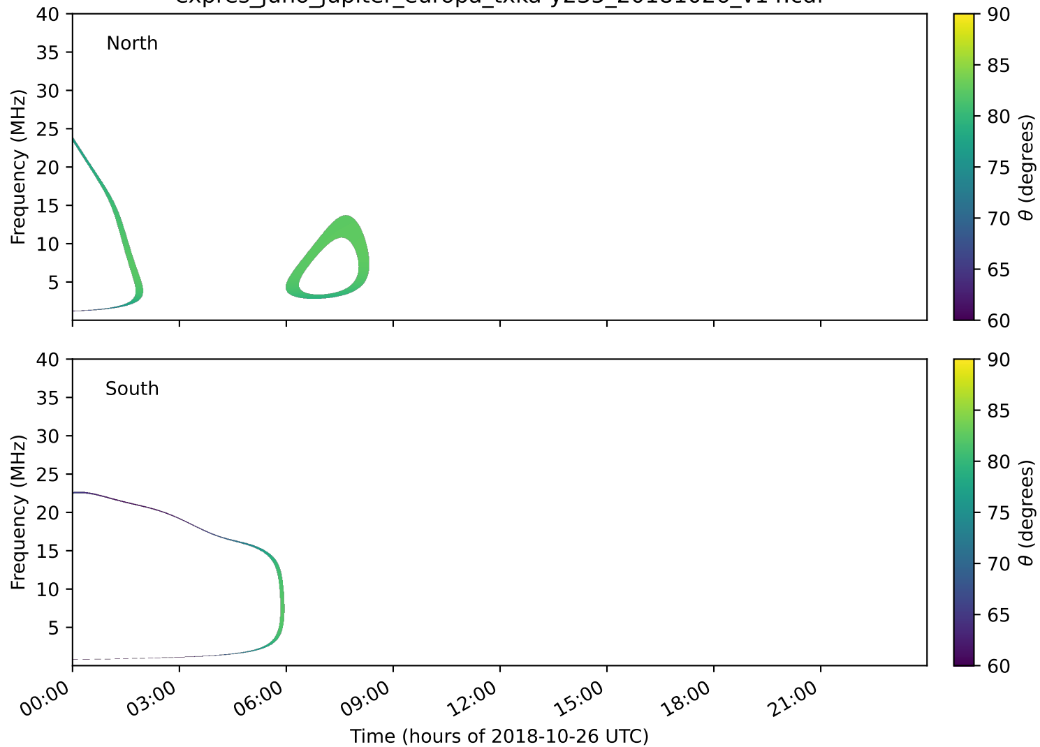
expres_juno_jupiter_europa_txka-y235_20181026_v14.cdf
