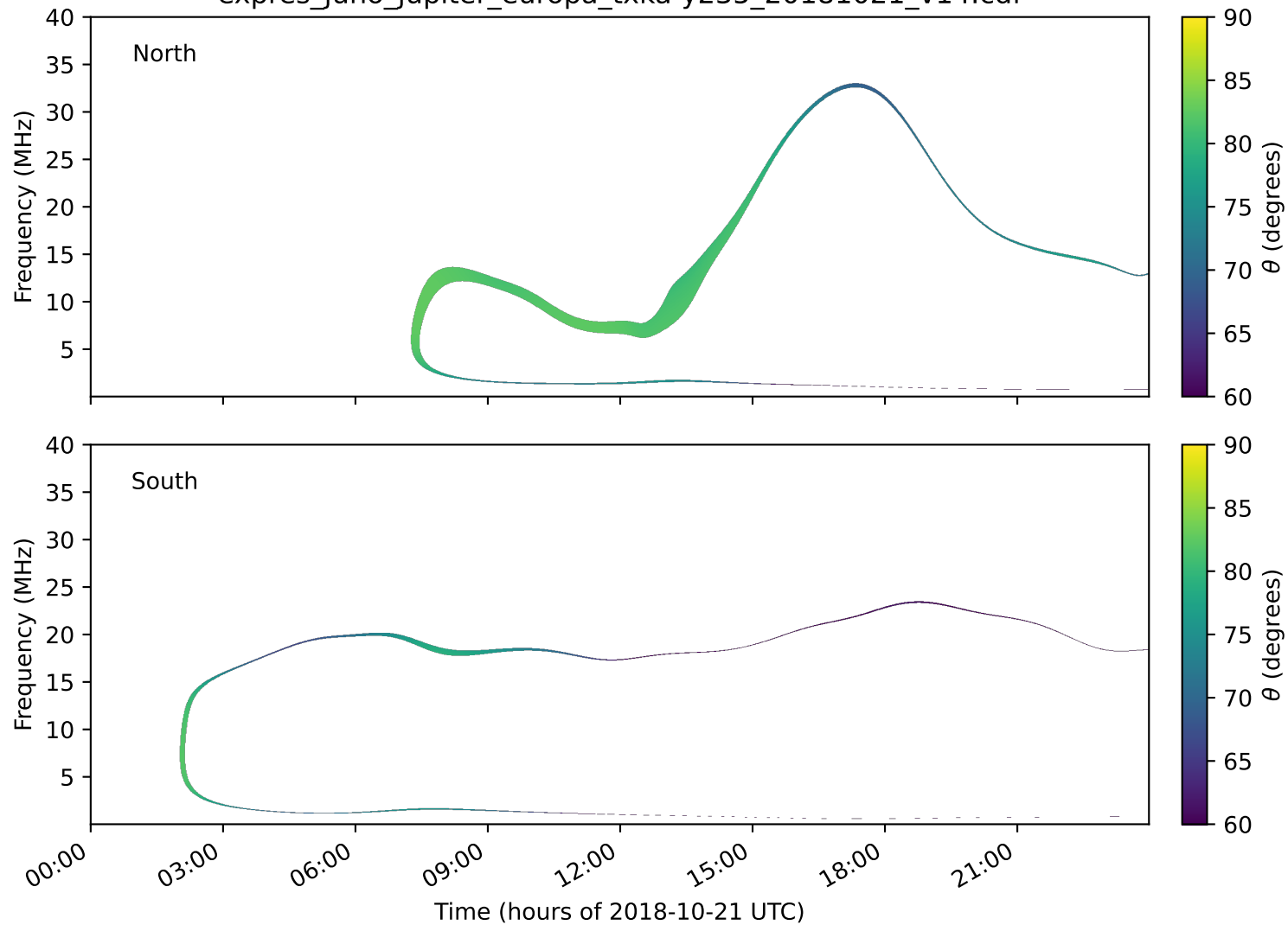
expres_juno_jupiter_europa_txka-y235_20181021_v14.cdf
