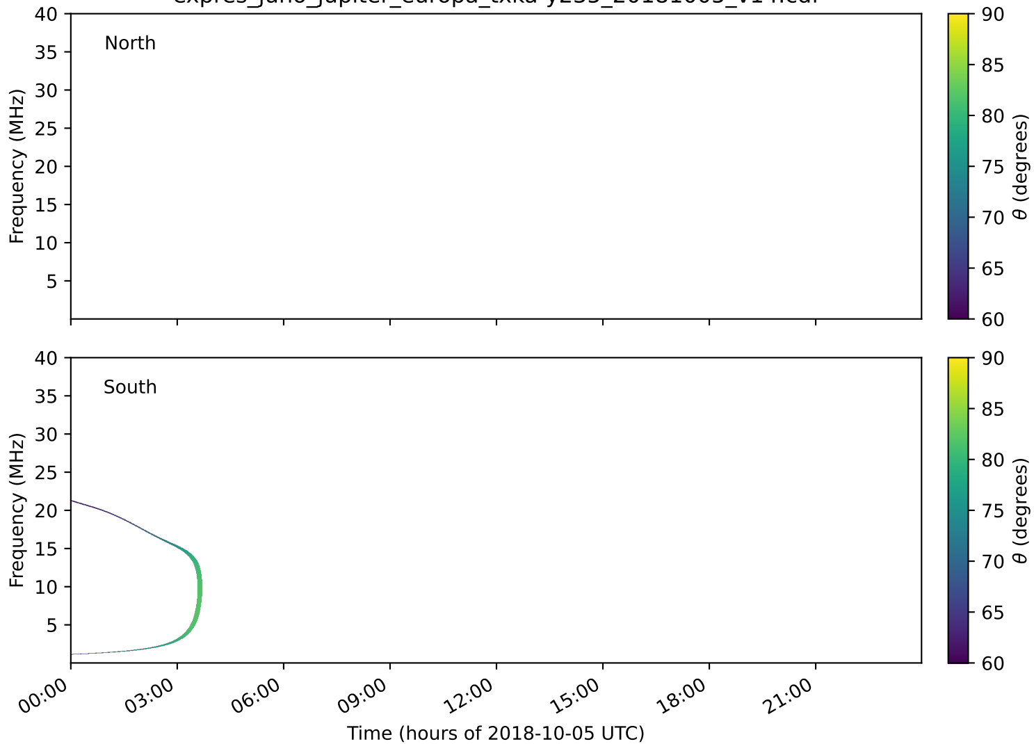
expres_juno_jupiter_europa_txka-y235_20181005_v14.cdf
