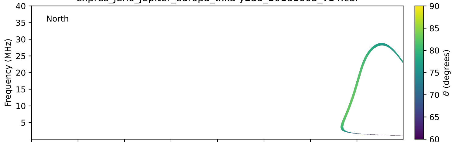
expres_juno_jupiter_europa_txka-y235_20181003_v14.cdf
