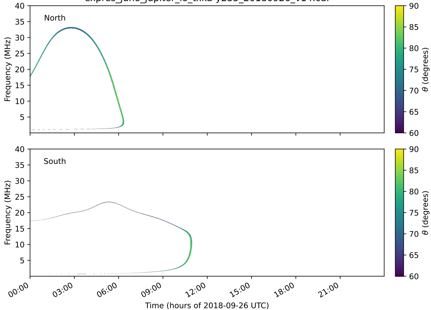
expres_juno_jupiter_io_txka-y235_20180926_v14.cdf
