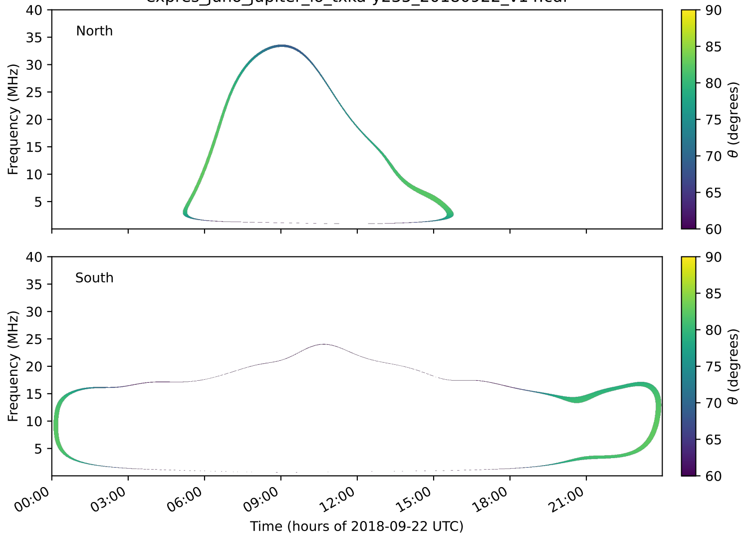
expres_juno_jupiter_io_txka-y235_20180922_v14.cdf
