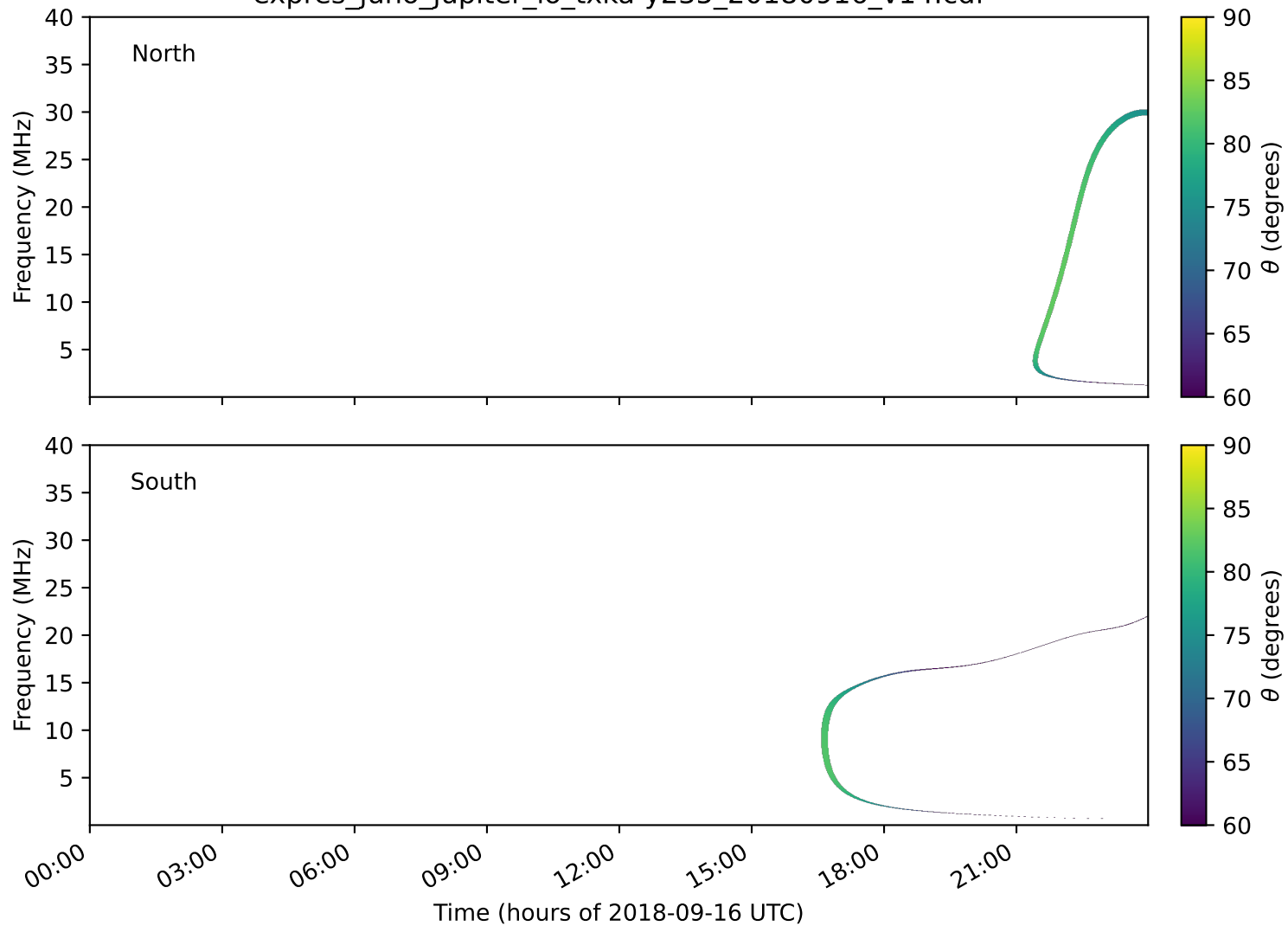
expres_juno_jupiter_io_txka-y235_20180916_v14.cdf
