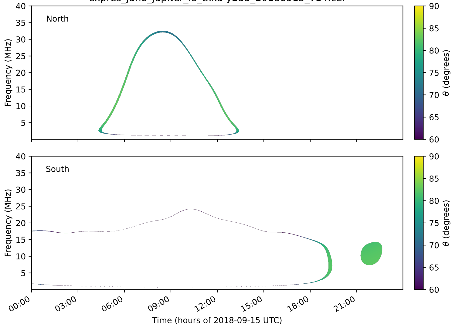
expres_juno_jupiter_io_txka-y235_20180915_v14.cdf
