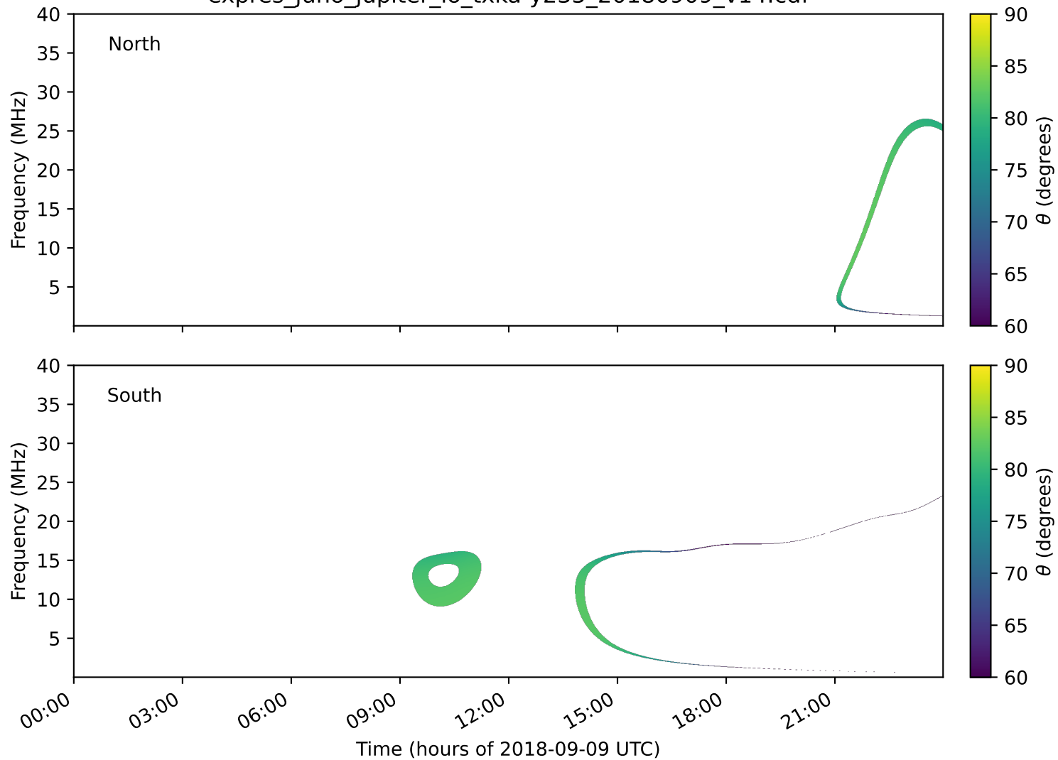
expres_juno_jupiter_io_txka-y235_20180909_v14.cdf
