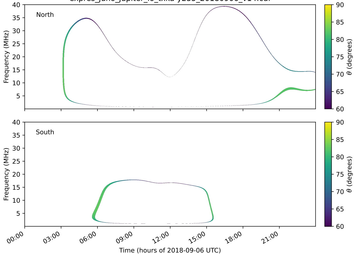
expres_juno_jupiter_io_txka-y235_20180906_v14.cdf
