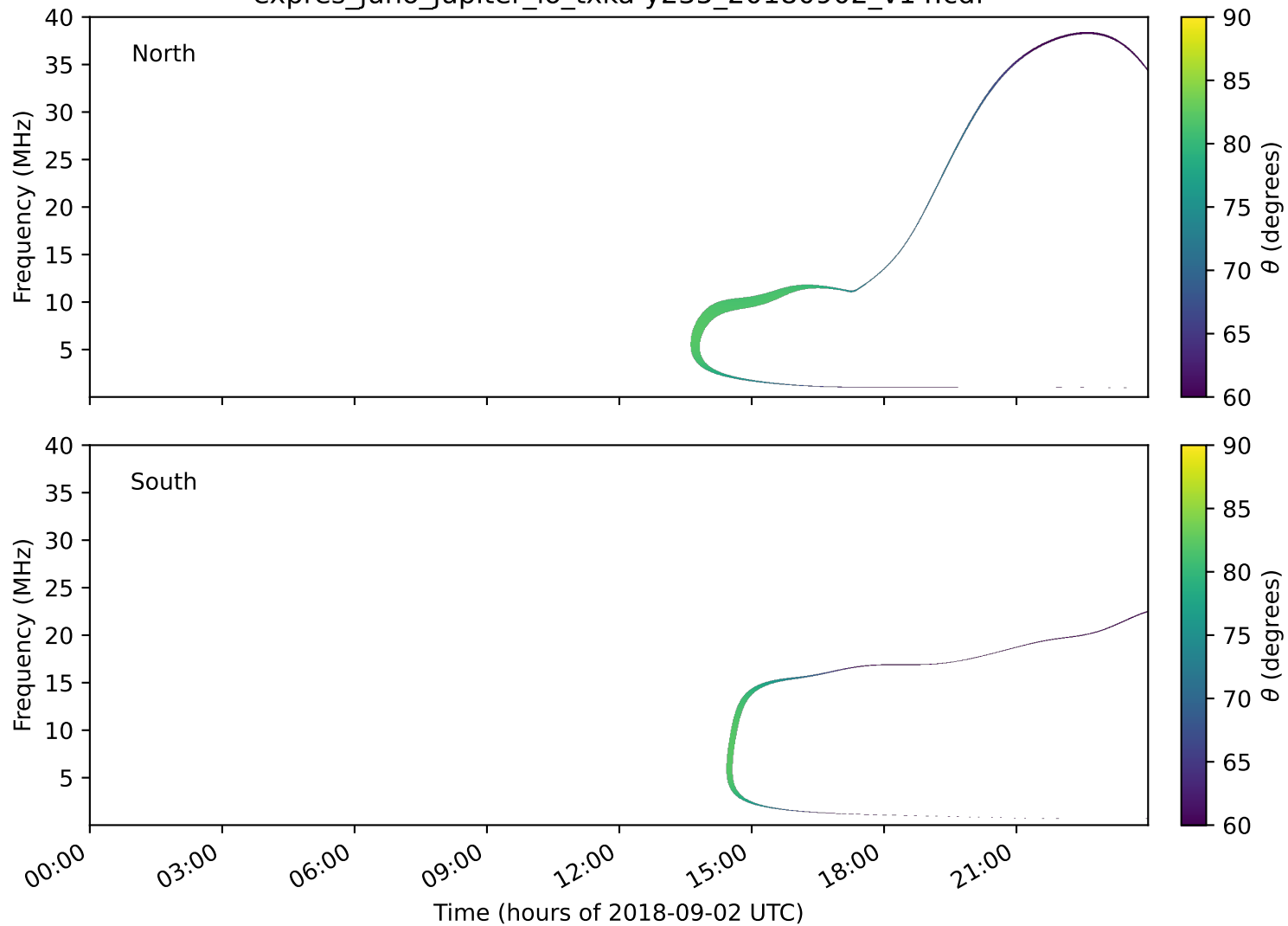
expres_juno_jupiter_io_txka-y235_20180902_v14.cdf
