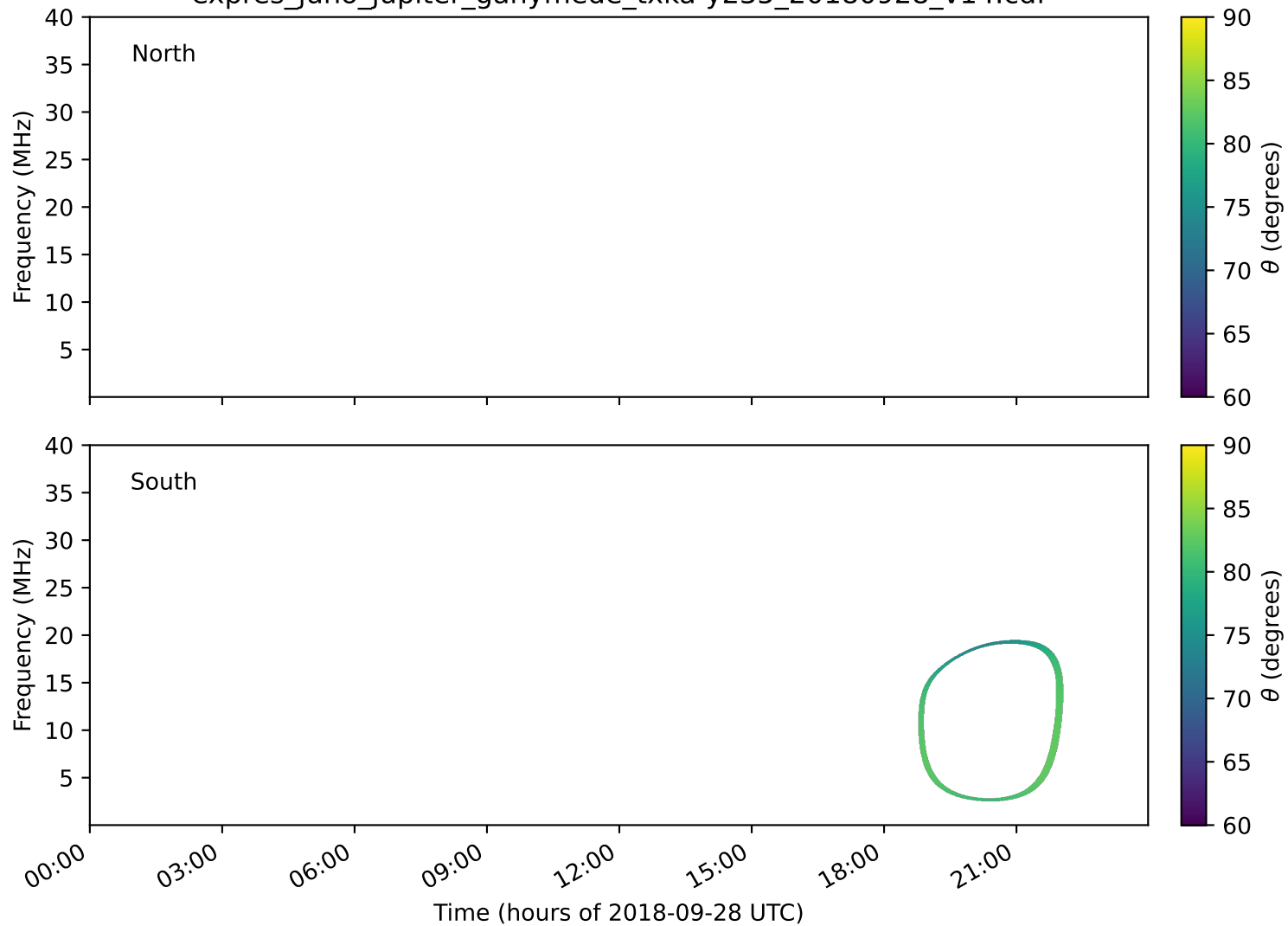
expres_juno_jupiter_ganymede_txka-y235_20180928_v14.cdf
